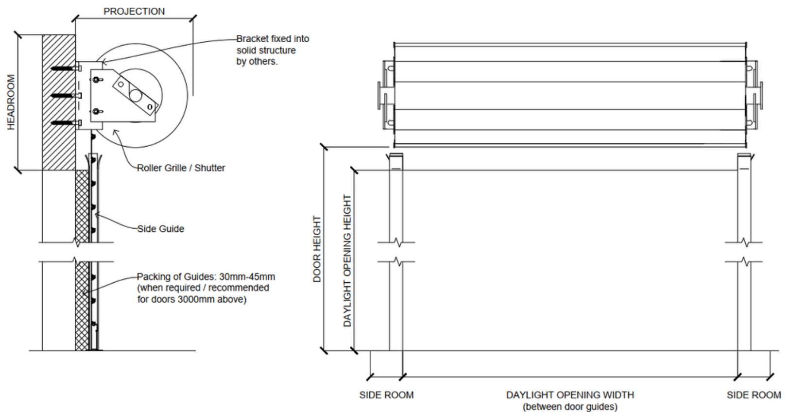
NOTE: Manual Door Operation drawn above (for illustration purposes only).
